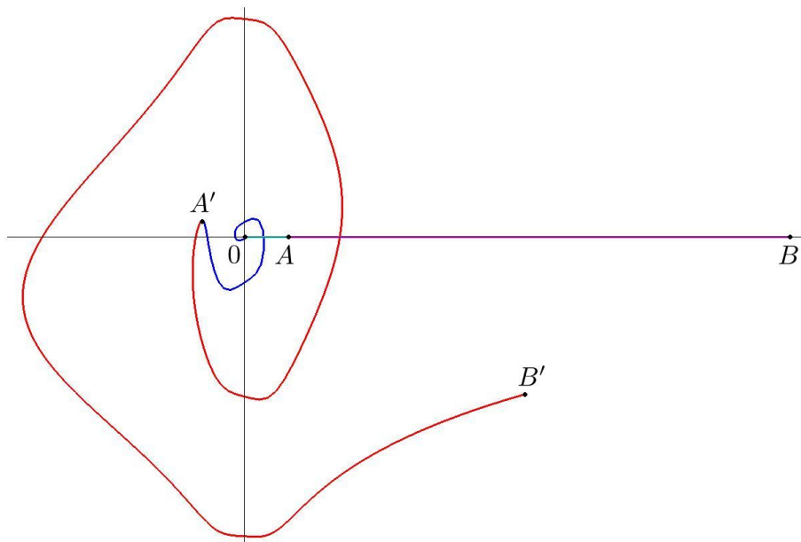
Figure 4.1: A numerical simulation describing the crucial geometrical features of supersublinear problems like (4.1). In particular, in the figure it is shown the manner in which a half-line from the origin is deformed by the Poincaré map \Psi associated with the planar Hamiltonian system x' = y, y' = -\lambda f(x) , for f(x) = \frac{4x^3}{1+x^4} and T = 1 . For the value \lambda = 50 , the positive x -axis is transformed into a double spiral winding around the origin. More precisely, the image of the segment \overline{0A} through \Psi is the small spiral-like arc connecting 0 to A' , while the image of the segment \overline{AB} is the large spiral-like arc connecting A' to B' . Notice that the six nontrivial intersections of \Psi(\overline{0B}) with the x -axis correspond to six nodal solutions to the Neumann problem associated with u'' + \lambda f(u) = 0 , starting with a positive initial value x(0) with (x(0), 0) \in \overline{0B} . Indeed, we have two solutions with respectively: one zero, two zeros, three zeros in ]0, T[ (exactly). For each pair of such solutions, one is with a “small” initial value (namely with (x(0), 0) \in \overline{0A} ) and the other is with a “large” initial value (namely with (x(0), 0) \in \overline{AB} ). Other six solutions can be obtained from initial points on the negative x -axis. The spiral will make more winds around the origin as \lambda grows, thus producing more pairs of solutions to the Neumann problem. Along the chapter, we will prove that such kind of geometry provides multiple pairs of T -periodic solutions, as well.
